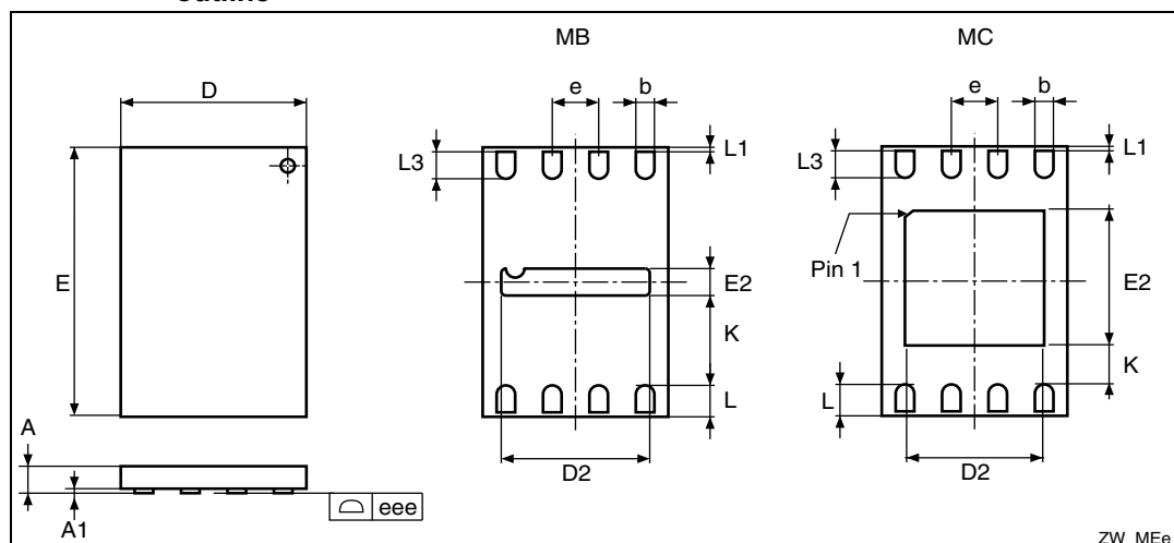
Figure 19. UFDFPN8 (MLP8) - 8-lead ultra thin fine pitch dual flat no lead, package outline
